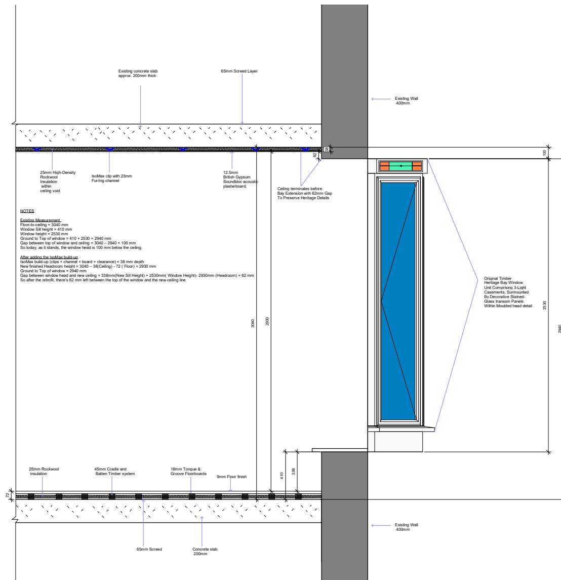
① Section of Bay window 1 : 10
