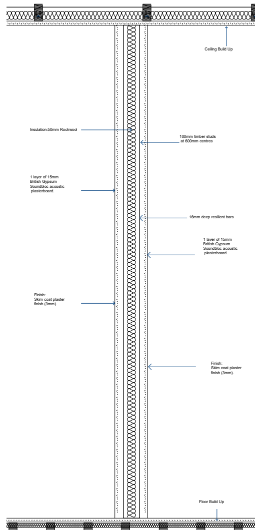
① Section of wall 1 : 7
