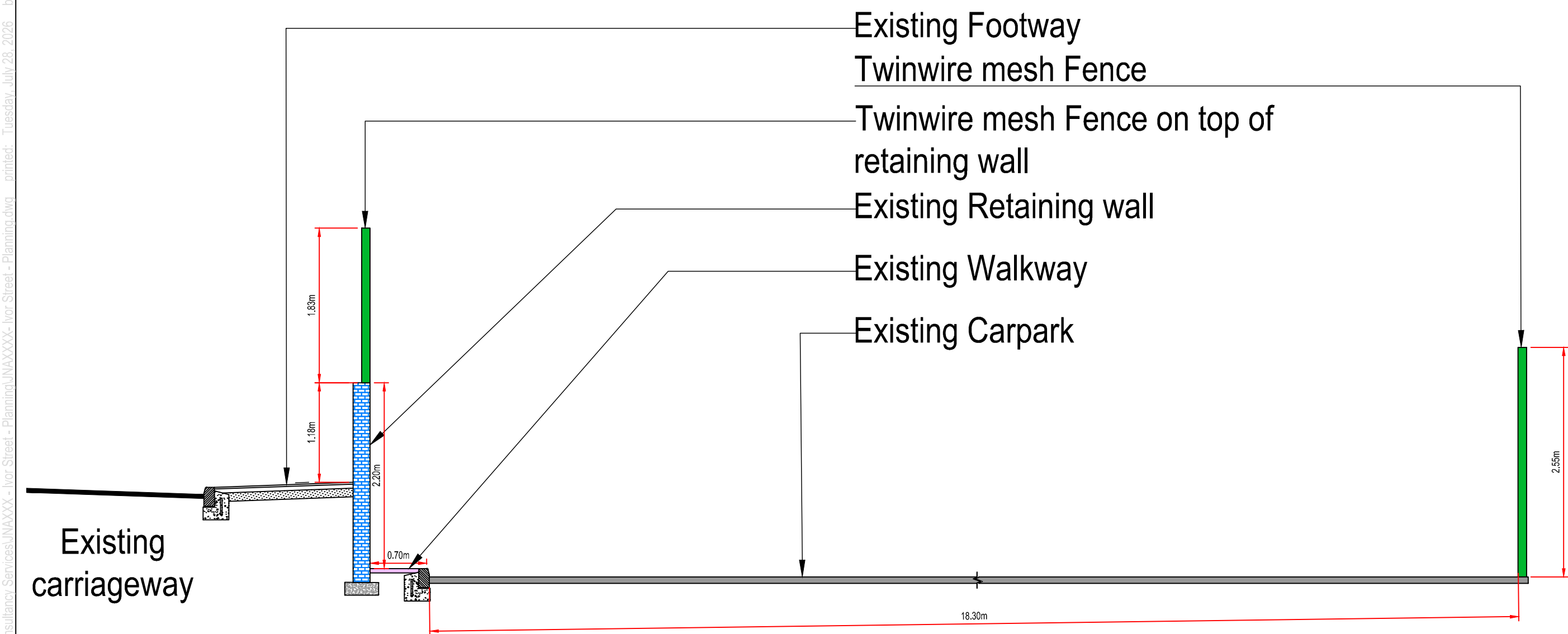
Twinwire fence panel Scale 1:50
