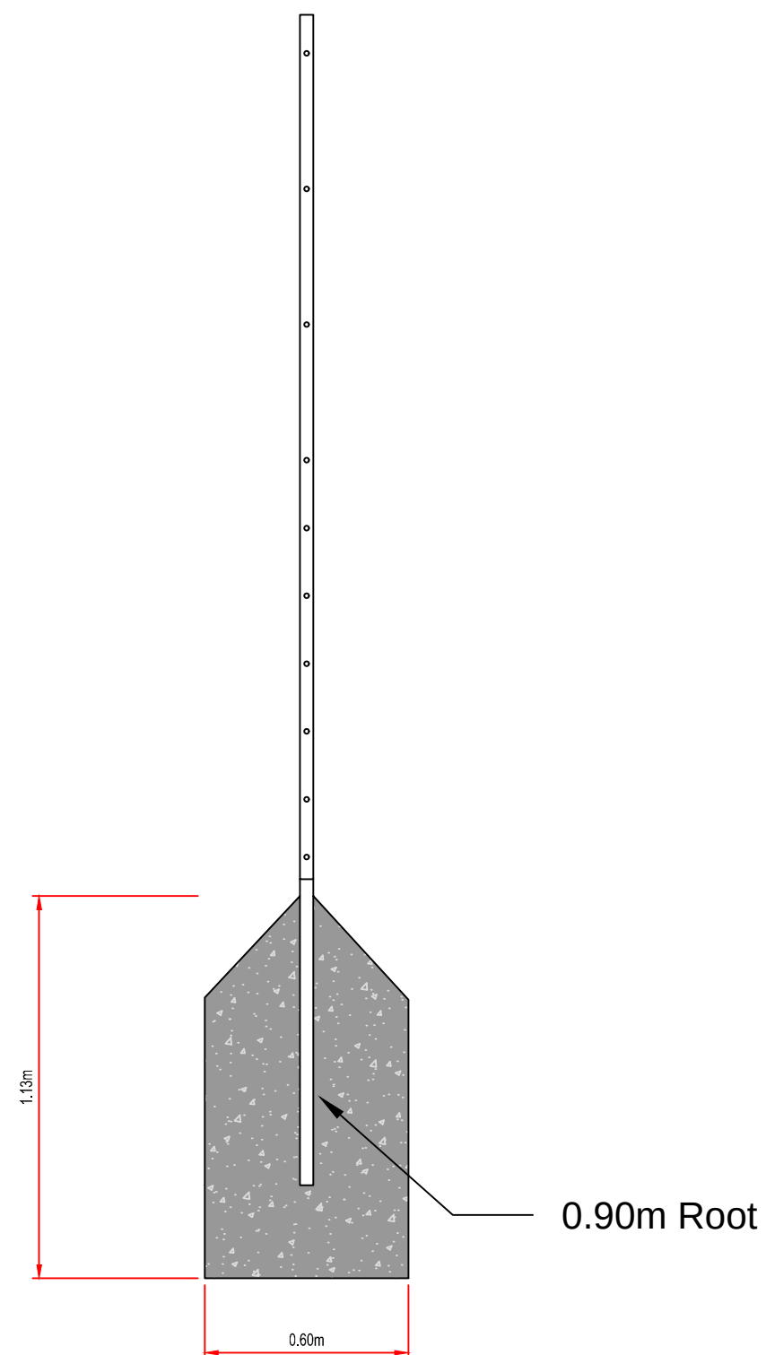
Foundation detail Scale 1:50
