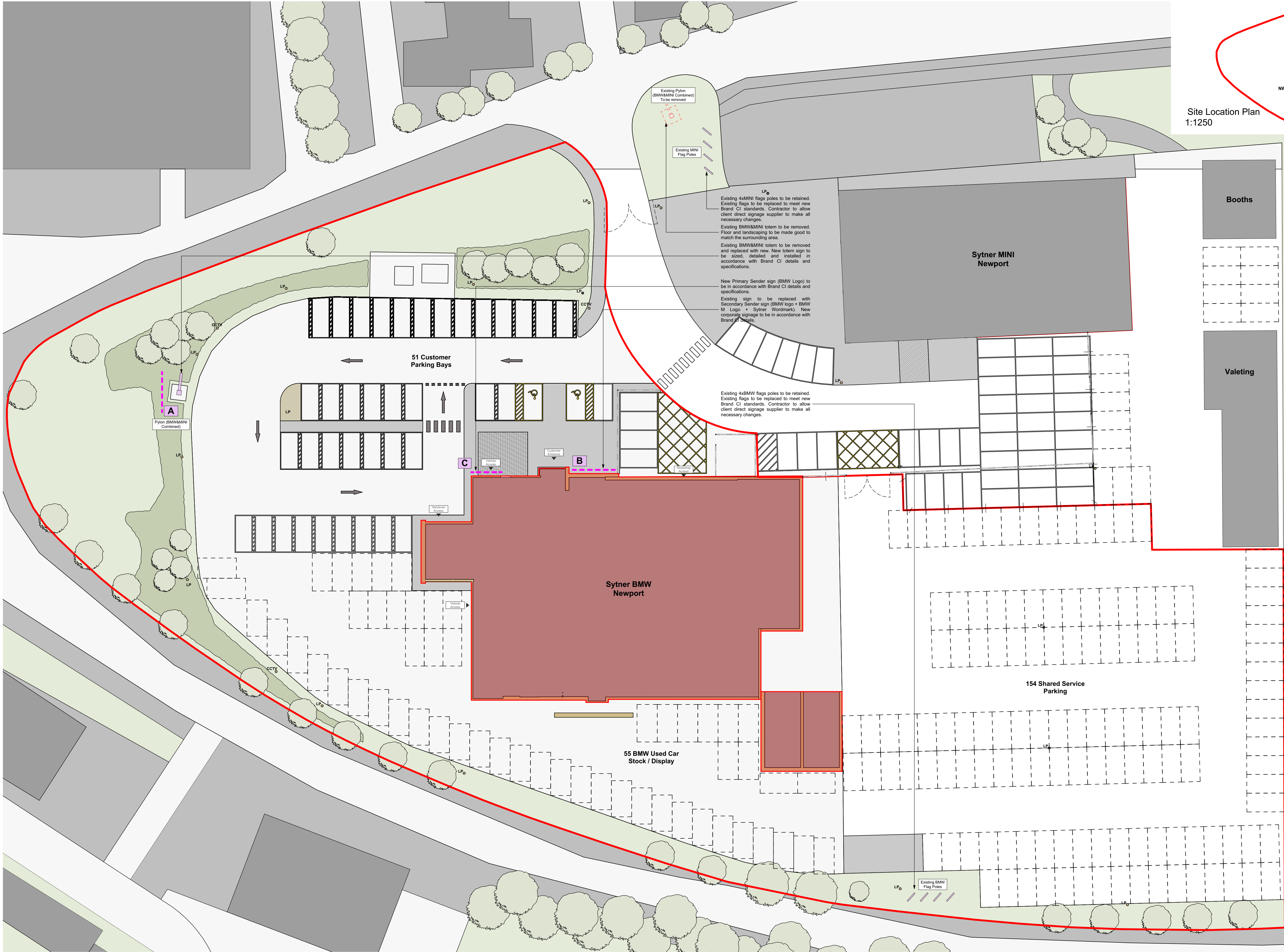
Proposed Site Plan BMW 1:250
