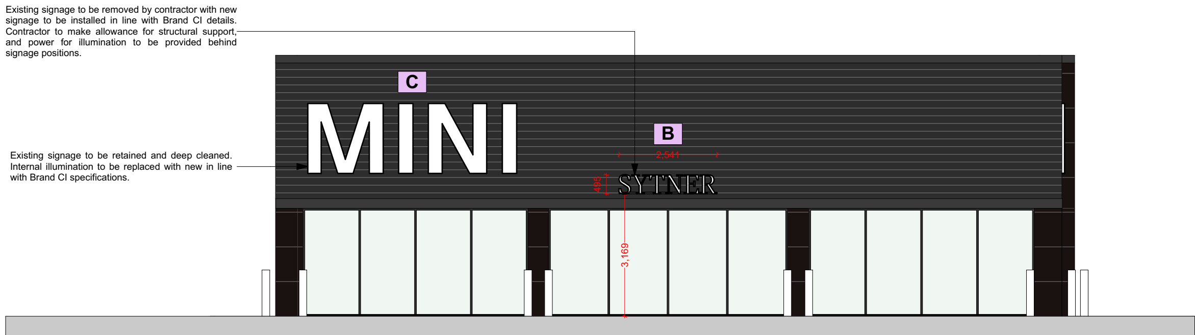
Proposed North West Elevation 1:100
