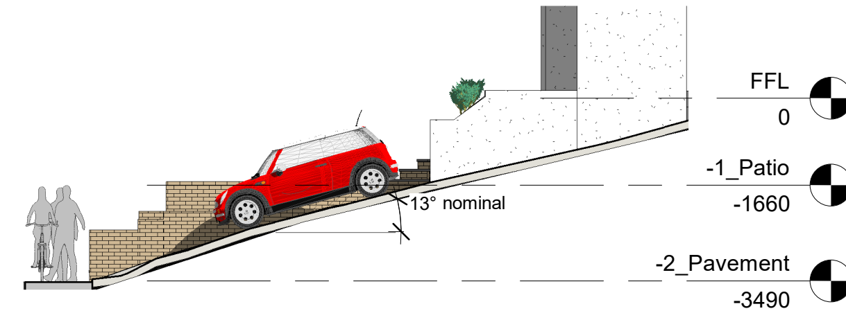
5 SIDE DRIVEWAY 1 : 100
