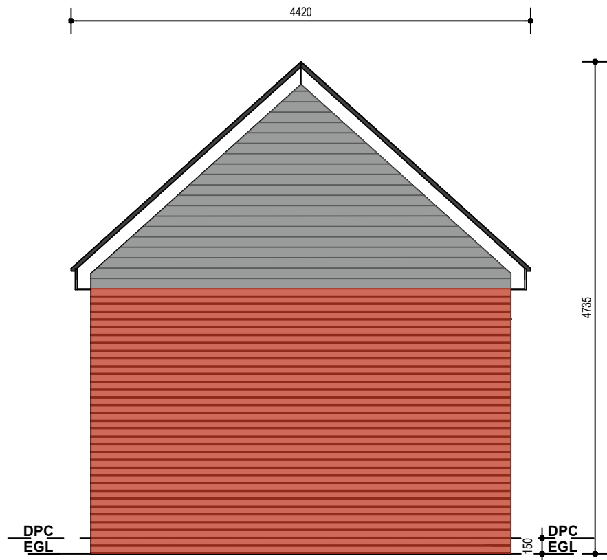
Rear Elevation
