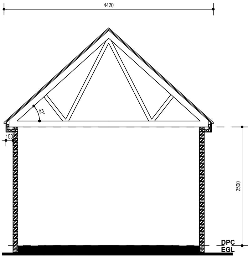
Section
