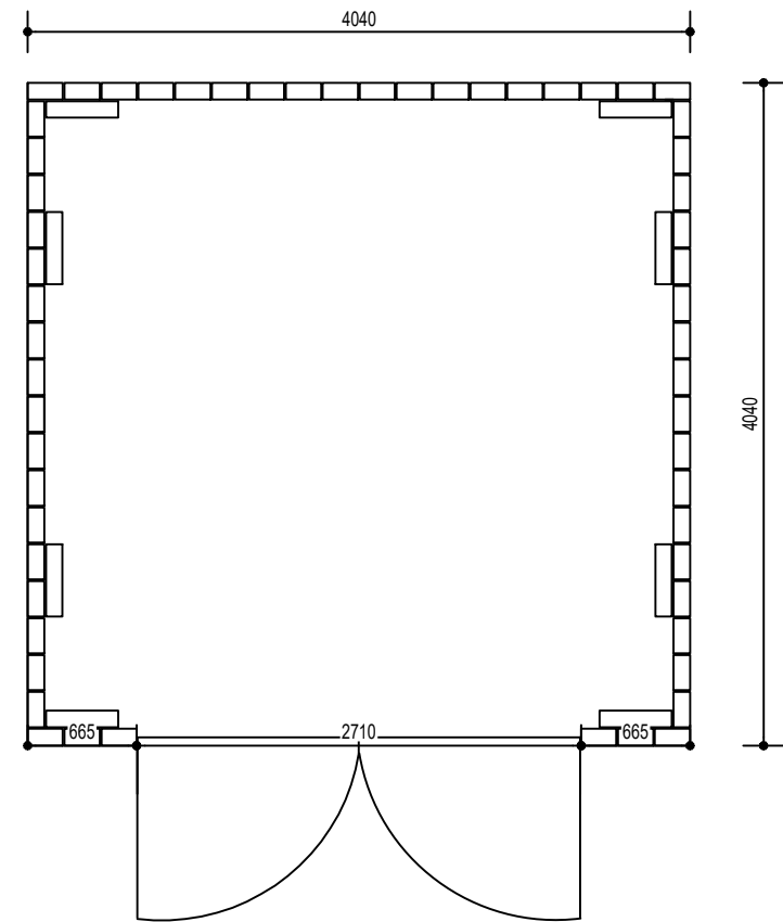
Floor Plan
