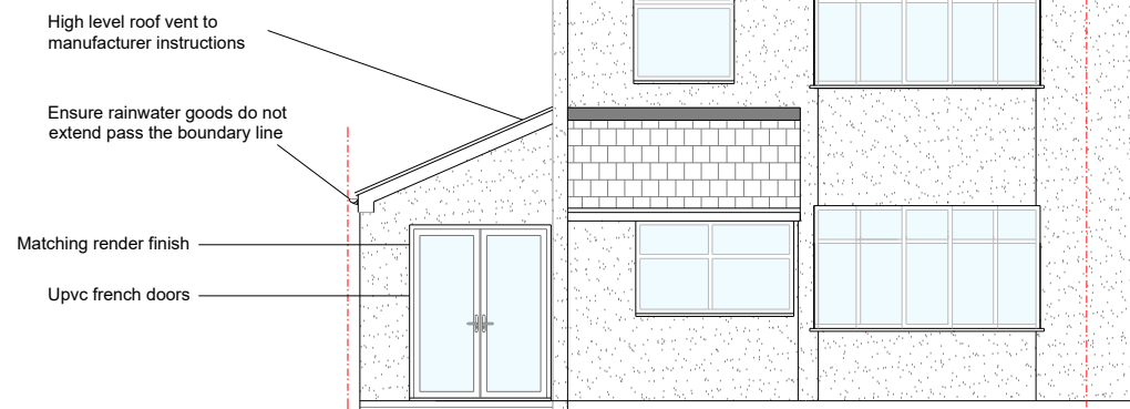
REAR ELEVATION
