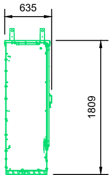
Left Elevation
