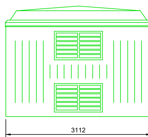
Rear Elevation
