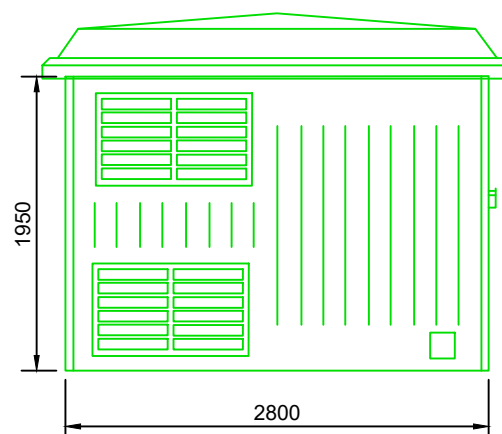
Left Elevation
