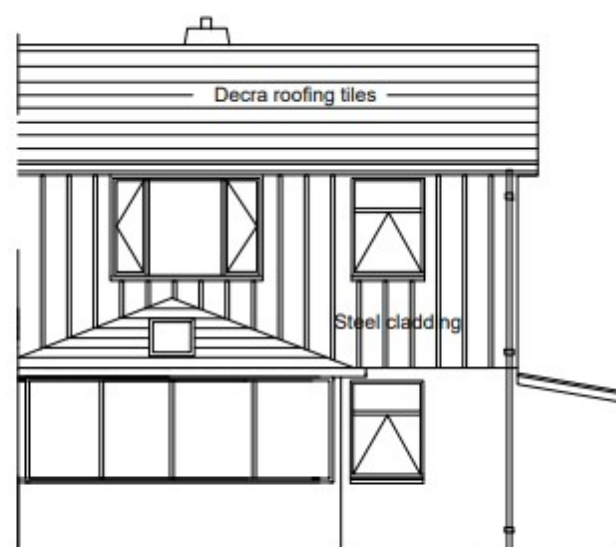
Rear elevation current
